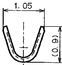
WIRE BARREL
