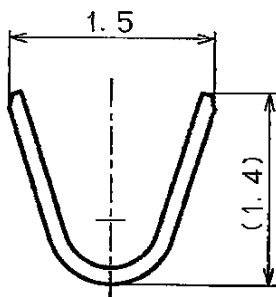
INSULATION BARREL
