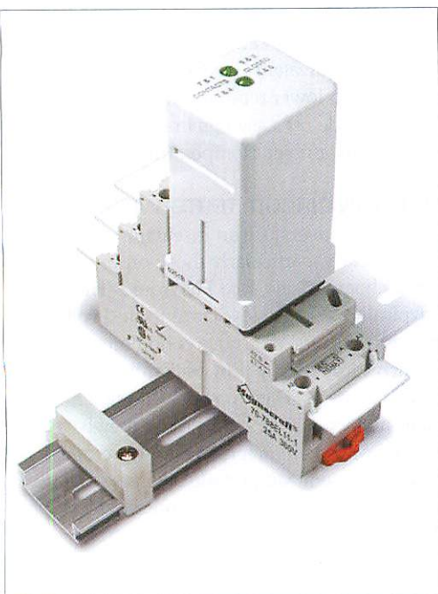
A sequencing relay changes state when a coil-driver circuit applies a pulse to its coil. This sequencing relay from Magnecraft includes LEDs on the top that indicate which contact pairs are closed. Courtesy of Magnecraft.
