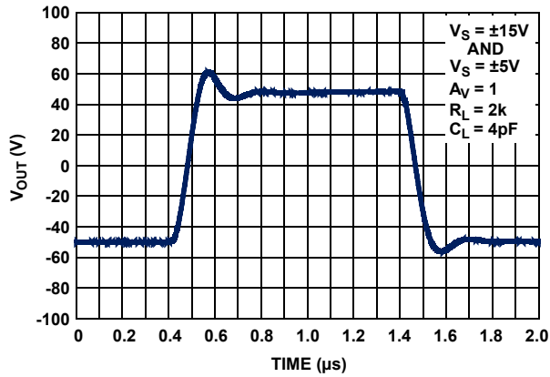
FIGURE 78. CHARACTERIZED SMALL-SIGNAL TRANSIENT RESPONSE
